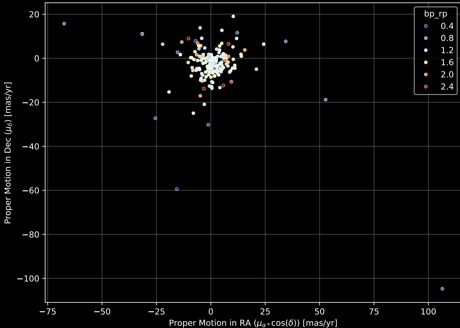
APOGEE DR17 Field: [162+34_btx] Proper Motion Diagram (n= 192)
