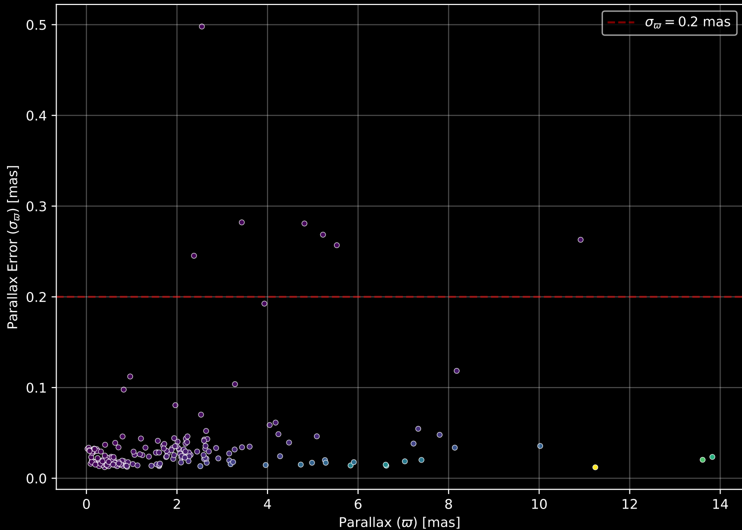
APOGEE DR17 Field: [162+34_btx] Parallax Quality (n= 192)
