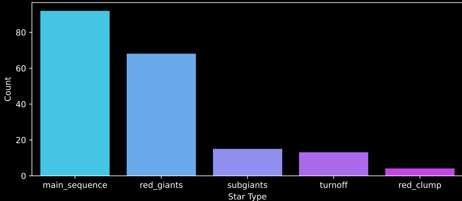
APOGEE DR17 Field: [162+34_btx] Count plot of Star Type
