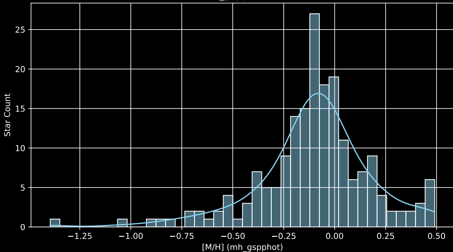
APOGEE DR17 Field: [162+34_btx [M/H] (mh_gspphot) (n= 191)
