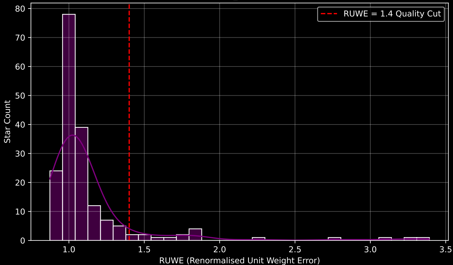
GAPOGEE DR17 Field [162+34_btx] RUWE Distribution (n= 182)
